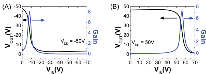
Figure 5. Transfer and gain characteristics of inverters constructed from unipolar p - and n -type PbSe NW FETs at (A) negative and (B) positive V_{DD} .
